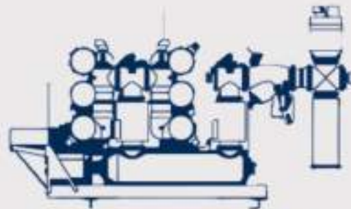
Gas Insulated Substation
